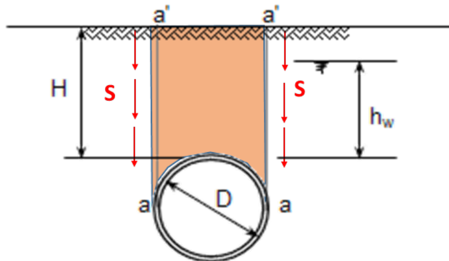
Plate A.2 Shear design case
